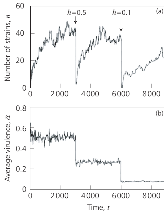
Figure 9.5 (a) The number n of pathogen strains present at time t , in the superinfection model, with mutations arising uniformly in the interval 0 \leq \alpha \leq 1 . At time t = 3\,000 , the total number of hosts h is decreased by 50%. The number n(t) subsequently increases again. At t = 6\,000 the number of hosts is reduced to 10% (since the rate of new mutants able to invade is 10% of the former value, the growth in n proceeds at a slower rate). (b) Corresponding average values of the virulence as a function of time. Removal of a fraction of the hosts permanently reduces the average virulence by that same fraction. Source: May and Nowak (1994).
