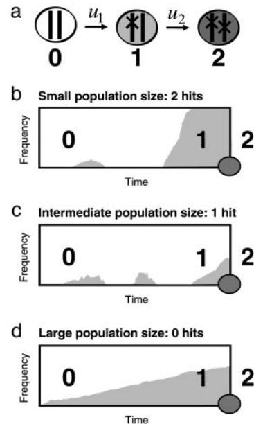
Fig. 1. Inactivating a TSG requires two, one, or zero rate-limiting steps depending on the population size. (a) Cells of type 0, 1, and 2 have, respectively, 0, 1, and 2 inactivated alleles of the TSG. The mutation rate for inactivating the first and second allele are given by u_1 and u_2 . Initially all cells are of type 0. (b) In small populations, N < 1/\sqrt{u_2} , type 1 cells will reach fixation before a cell of type 2 has been generated. The resulting kinetics have two rate-limiting steps (Eq. 1). (c) In intermediate populations, 1/u_1 < N < 1/\sqrt{u_2} , a lineage of type 1 cells generates a type 2 cell before reaching fixation. The resulting kinetics have one rate-limiting step (Eq. 2). (d) In large populations, 1/u_1 < N , type 1 cells are generated immediately and accumulate as a linear function of time. After some (short) time a type 2 cell will be generated. The kinetics involve two steps, none of which is rate-limiting for overall cancer progression (Eq. 3). This classification allows us to analyze the effect of cell number and mutation rate on the kinetics of TSG inactivation.
