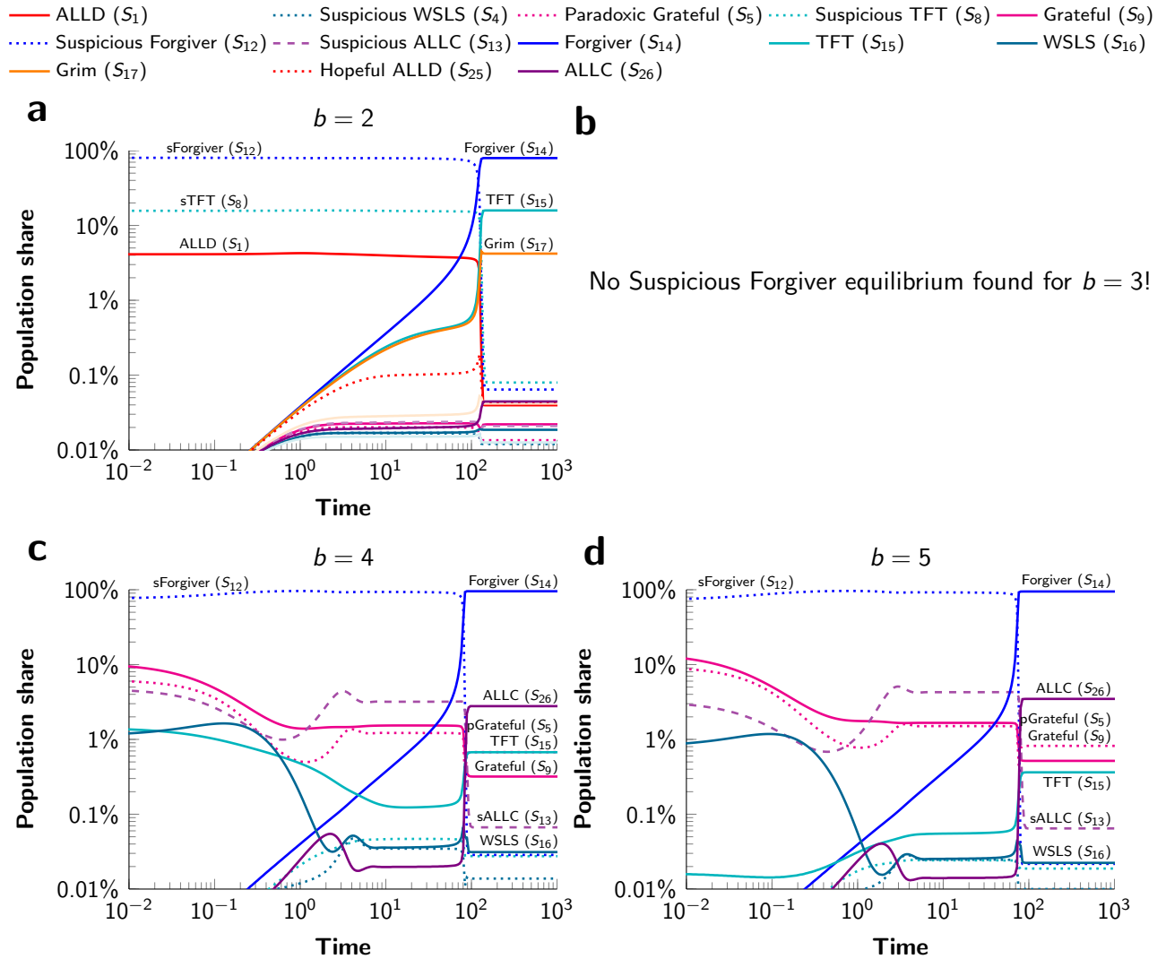
Figure S7: The Suspicious Forgiver equilibrium is unstable. In all panels, the simulations start from the mixed Suspicious Forgiver equilibrium. Small mutation rates can lead to the evolution of Forgiver due to its slightly higher payoff against cooperative strategies. If the mutation rate is sufficiently high, the simulation dynamics converge to the stable mixed Forgiver equilibrium. The error rate \epsilon is set to 5%, the number of rounds per game is L = 100 , and the mutation rate is u = 1\% .
