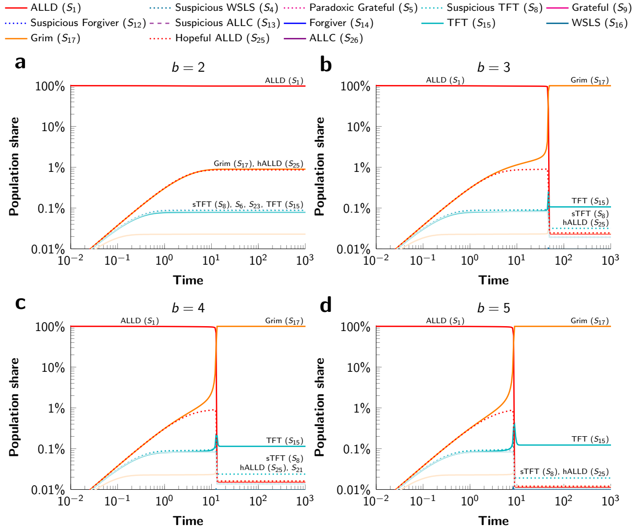
Figure S6: The ALLD equilibrium becomes unstable for high mutation rates. High mutation rates can lead to the evolution of Grim due to its higher payoff against cooperative strategies. If the mutation rate and the benefit value are sufficiently high, Grim outperforms ALLD and the simulation dynamics converge to a stable Grim equilibrium (panels b, c, and d). For smaller mutation rates or benefit values Grim cannot invade ALLD (panel a). In all panels, the simulations start from pure ALLD ( x_1 = 1 ). The error rate \epsilon is set to 5%, the number of rounds per game is L = 100 , and the mutation rate is u = 10\% .
