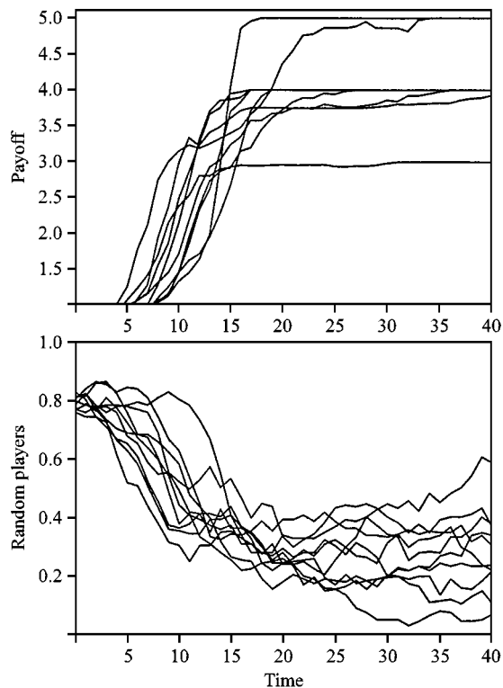
FIG. 6. It is better to learn from your parents than from random members of the population. The simulation compares the performance of two different strategies: (i) individuals who learn the language of their parents; and (ii) individuals who learn the language of an arbitrary member of the community (so called “random players”). The population size is 200. Initially 80% of the population are random players. The figure shows the increase in the average payoff as the community evolves a common language and the decrease of the fraction of random players. Note that the frequency of random players decline as long as the population is in the state of improving its language; once everyone speaks the same language there is no longer a difference in the performance of the two strategies (and random drift will eventually drive one of them to extinction). Parameters: n = 5 , m = 5 , every individual samples one other individual once (i.e. K = 1 and k = 1 ), 10 runs are shown.
