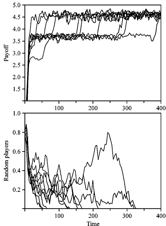
FIG. 7. Take advantage of mistakes. The possibility of errors during language acquisition enables the system to reach the global optimum. Furthermore, such errors introduce a consistent selection pressure against the random players. The figure shows 10 simulation for exactly the same parameter values as in Fig. 4. The only difference is that individuals can make mistakes while learning the language: with probability \rho , the response of another individual to a particular object is mistaken for another (randomly chosen) response. We use \rho = 0.01 . In 10 of 10 runs, the random players become extinct and the population converges to the maximum payoff were each object is associated with exactly one signal and vice versa.
