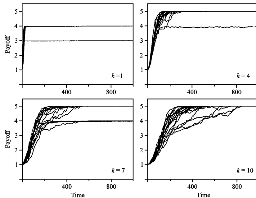
FIG. 2. A common language evolves if children learn their language from individuals in the previous generation who have a high payoff. There are N = 100 individuals communicating about n = 5 objects using (up to) m = 5 signals. There are discrete generations. In one generation each individual is talking to every other individual. The payoffs of all interactions are summed up. Each individual of the next generation chooses K individuals of the previous generation and samples their responses (1 response per object per individual is sampled). P and Q are derived from A . The probability that an individual is chosen for being sampled is proportional to its payoff in the language game. Thus successful individuals have a higher chance of passing on their language. The four panels show 20 runs each for K = 1, 4, 7, 10 . All simulations eventually settle to binary P matrices achieving payoffs 6, 8, or 10. The case K = 1 has the fastest convergence to a common language but reaches on average a slightly lower final payoff. K = 10 has slowest convergence, but reaches this maximum payoff in 20 of 20 cases. This is, however, a coincidence. In simulations using 100 runs per K -value, there is no significant difference between K = 4, 7 or 10 , although K = 1 performs clearly worse.
