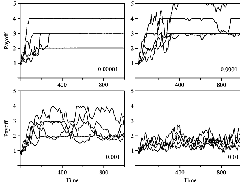
FIG. 5. Increasing amounts of noise make random sampling ineffective. Here the simulations of Fig. 3 are repeated for \rho = 0.00001, 0.0001, 0.001 and 0.01 . For small values of \rho the system manages to converge to a common language (which is represented a randomly chosen binary active matrix). For larger values of \rho the population no longer converges to a common language. Thus errors during language acquisition have very different effects on systems where individuals sample their parents (or other individuals with high payoff) as opposed to systems where individuals sample randomly chosen individuals. Five runs are shown for each value of \rho . For all runs we have K = 1 .
