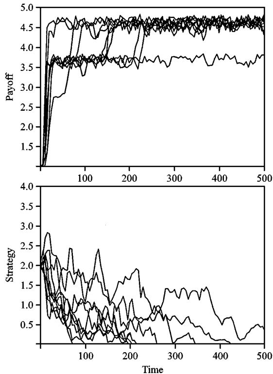
FIG. 8. In the presence of errors, is it better only to acquire the language from the parents or acquire the language from the parents and some other, randomly chosen individuals? Strategy, M , denotes the number of individuals that are sampled in addition to the parents. That is, every individual samples its parents and M other individuals of the previous generation. In our simulation, M varies from 0 to 4. In 10 out of 10 runs the average strategy of the population eventually converges to 0. In all runs the average payoff eventually converges to its maximum value. Same parameters as in Fig. 5.
