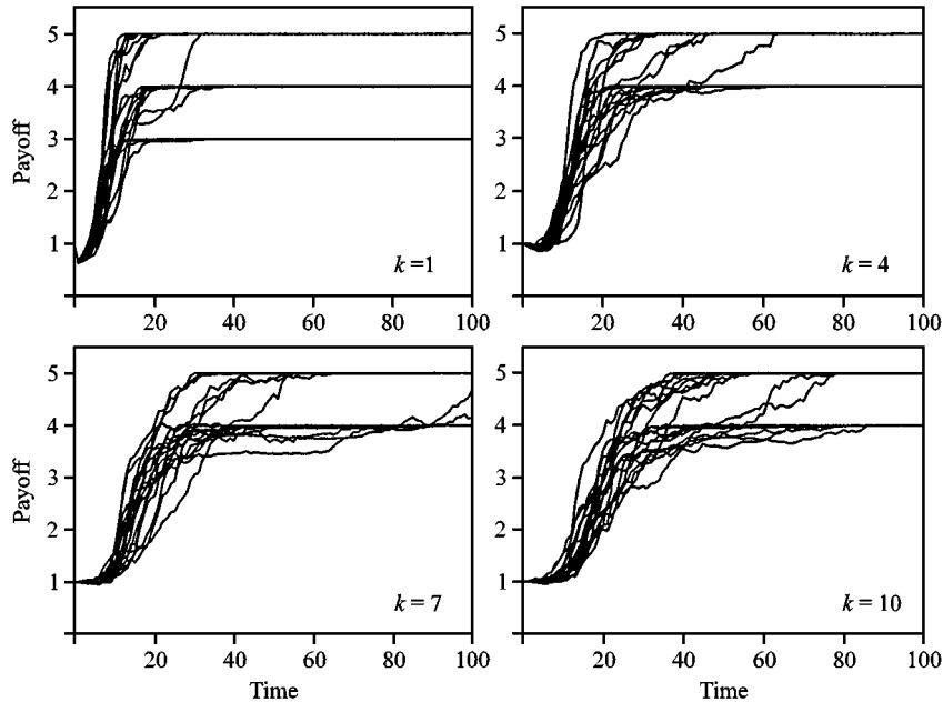
FIG. 1. A common language evolves if individuals with a high payoff in the language game produce more offspring and if children learn the language of their parents. There are N = 100 individuals communicating about n = 5 objects using (up to) m = 5 signals. There are discrete generations. In one generation each individual is talking to every other individual. The payoffs of all interactions are summed up. Individuals produce offspring for the next generation proportional to their total payoff. Offspring sample the active matrix from their parents thereby forming their own association matrix, A , between objects and signs. For each object, k responses are sampled. Individuals derive their P and Q from their A . Initially, every individual has a random A ; a_{ij} are taken from a uniform distribution on the interval (0, 1) . The four panels show 20 runs each for k = 1, 4, 7, 10 . All simulations eventually settle to binary P matrices achieving payoffs 6, 8, or 10. The case k = 1 has the fastest convergence to a common language but reaches on average a slightly lower final payoff than k = 4, 7, 10 .
